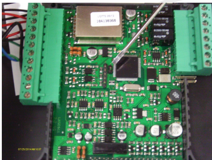
Jumper Location
