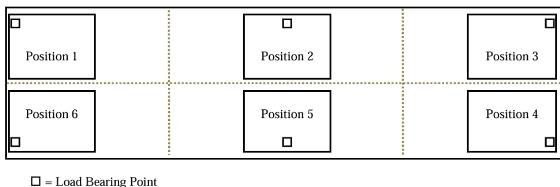
Figure 2. Prescribed Test Patterns for Combination Application Scales with More Than Two Sections
